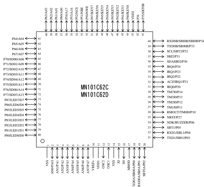
LQFP080-P-1414A *Pb free
