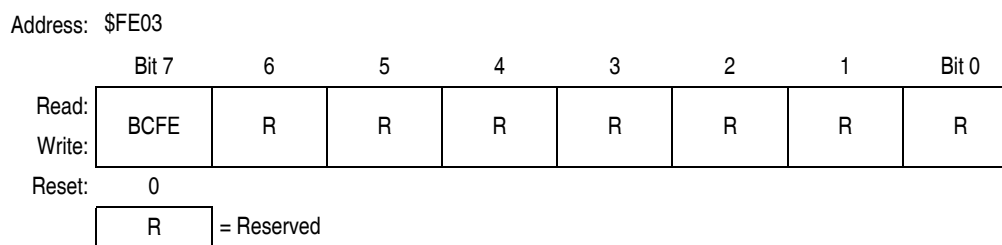
Figure 19-8. Break Flag Control Register (BFCR)
