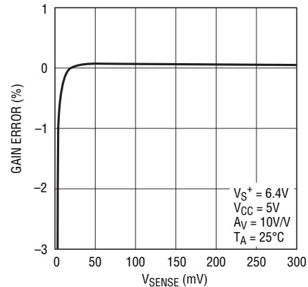
Gain Error vs VSSENSE
