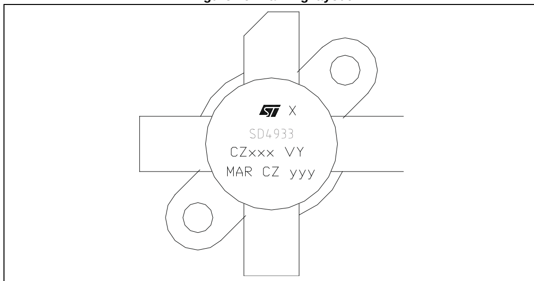
Figure 16. Marking layout
