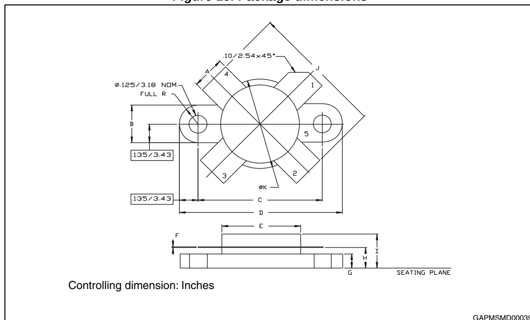
Figure 15. Package dimensions
