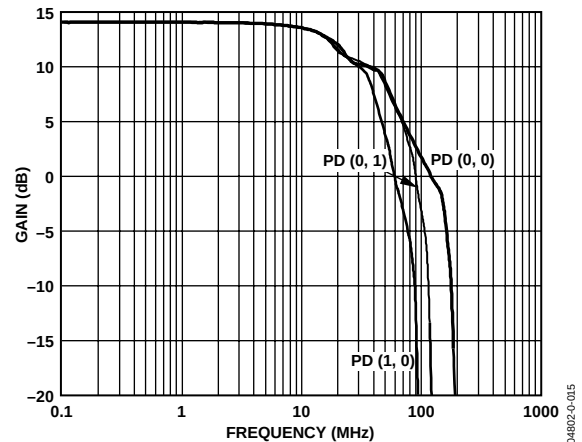
Figure 15. Large Signal Frequency Response Quad Op Amp Circuit (Figure 29) V_S = \pm 5\text{ V} , R_{LOAD} = 100\ \Omega , G = +5 , V_{OUT} = 4\text{ V p-p}
