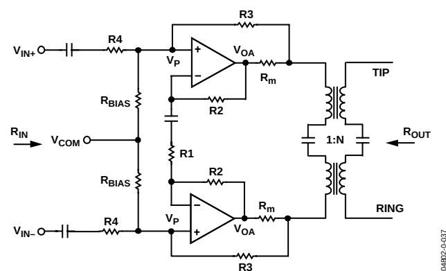
Figure 37. Typical ADSL/ADSL2+ Application Circuit
