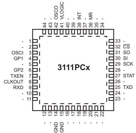
44 Pin Plastic QFN, 7mm x 7mm
