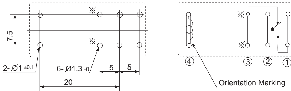
I PC Board mounting hole layout (BOTTOM VIEW)
