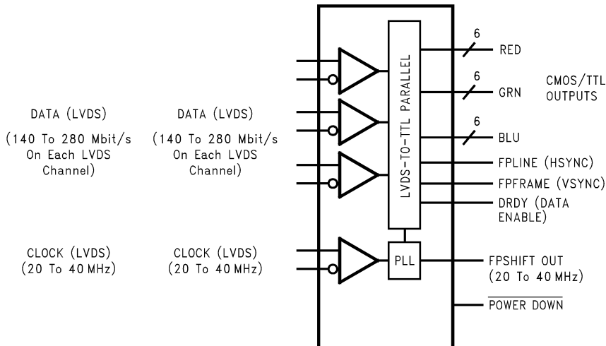
Figure 2. DS90CR562 See Package Number DGG
