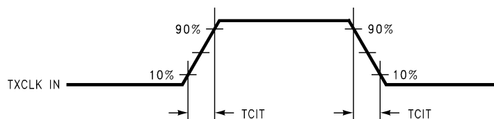
Figure 10. DS90CR561 (Transmitter) Input Clock Transition Time
