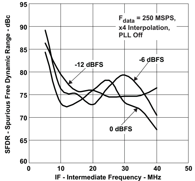
Figure 6. In-Band SFDR vs IF
