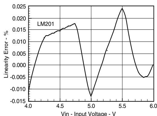
Fig. 20 Linearity Error vs. Input Voltage
