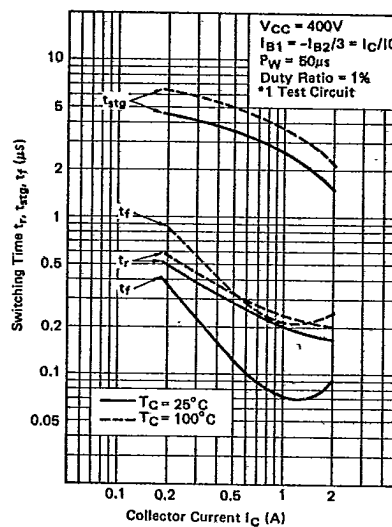
SWITCHING TIME
