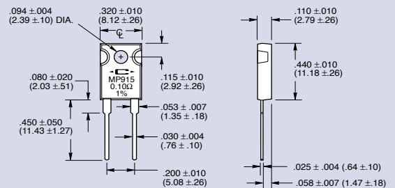
Figure 1 TO-126 Style MP915
