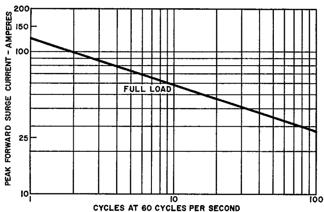
MAXIMUM NON-REPETITIVE MULTICYCLE FORWARD SURGE CURRENT
