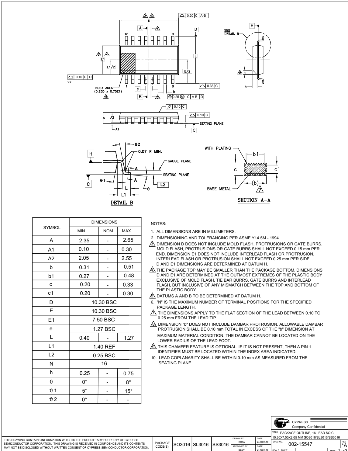
Figure 40. SOIC 16-Lead, 300-mil Body Width (SO3016)
