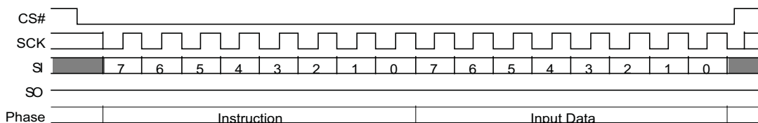
Figure 55. Bank Register Write (BRWR 17h) Command
