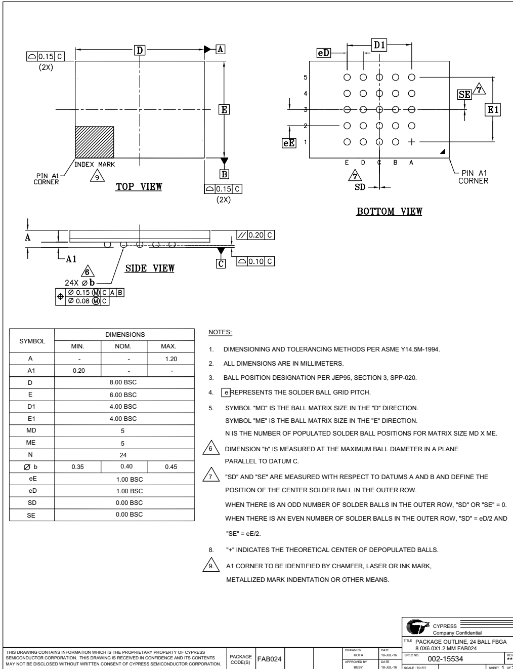
Figure 42. Ball Grid Array 24-Ball 6x8 mm (FAB024)
