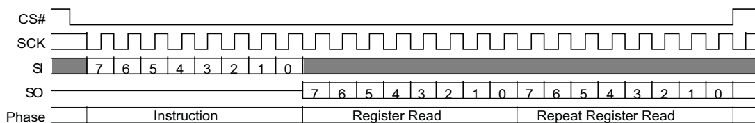
Figure 54. Read Bank Register (BRRD 16h) Command
