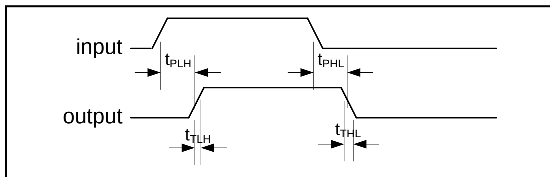
Figure 2. AC Waveforms
