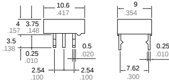
Self-clinching terminal
