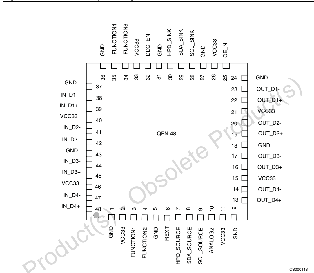
Figure 5. STHDLS101T pin configuration
