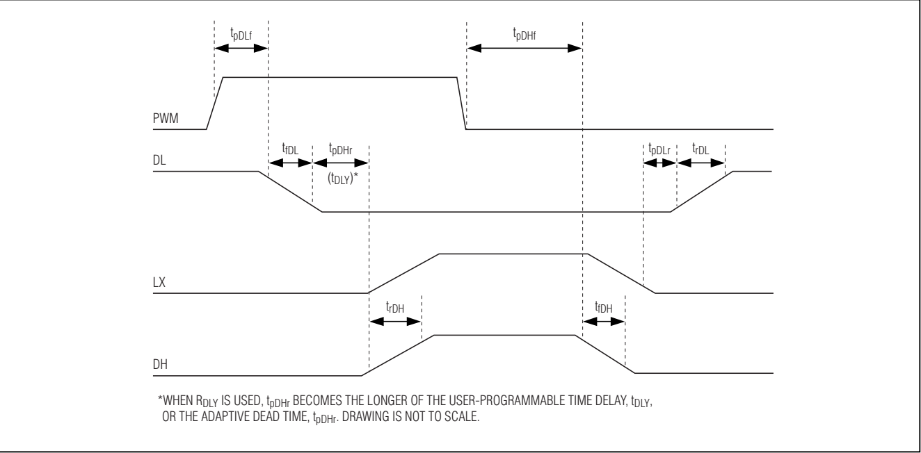
Timing Diagram
