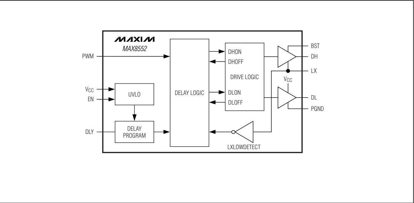
Functional Diagram
