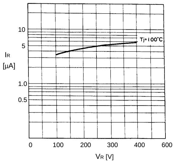
Reverse characteristics
