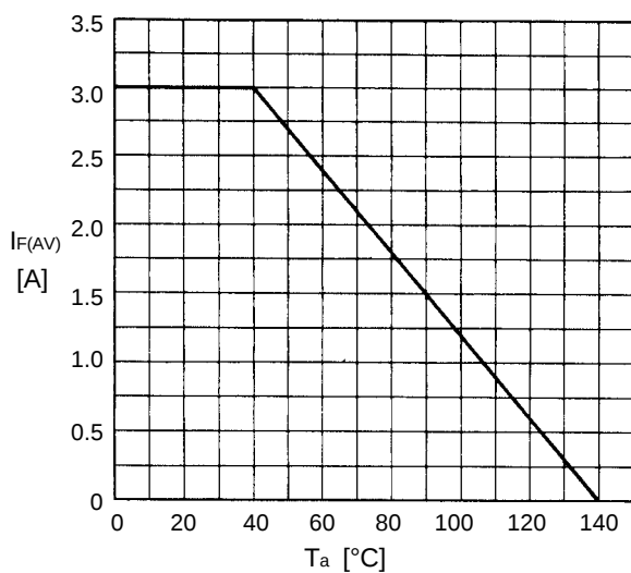
Current derating ( I_{F(AV)}-T_a )
