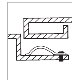
Rivet Mount
