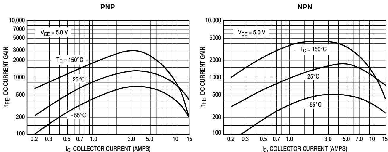
Figure 6. DC Current Gain
