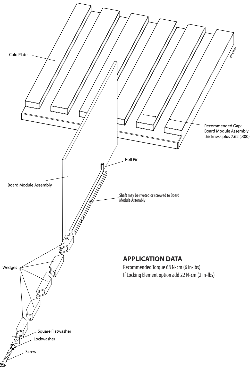
Series 260 "Card-Lok" Retainer (cold plate)
