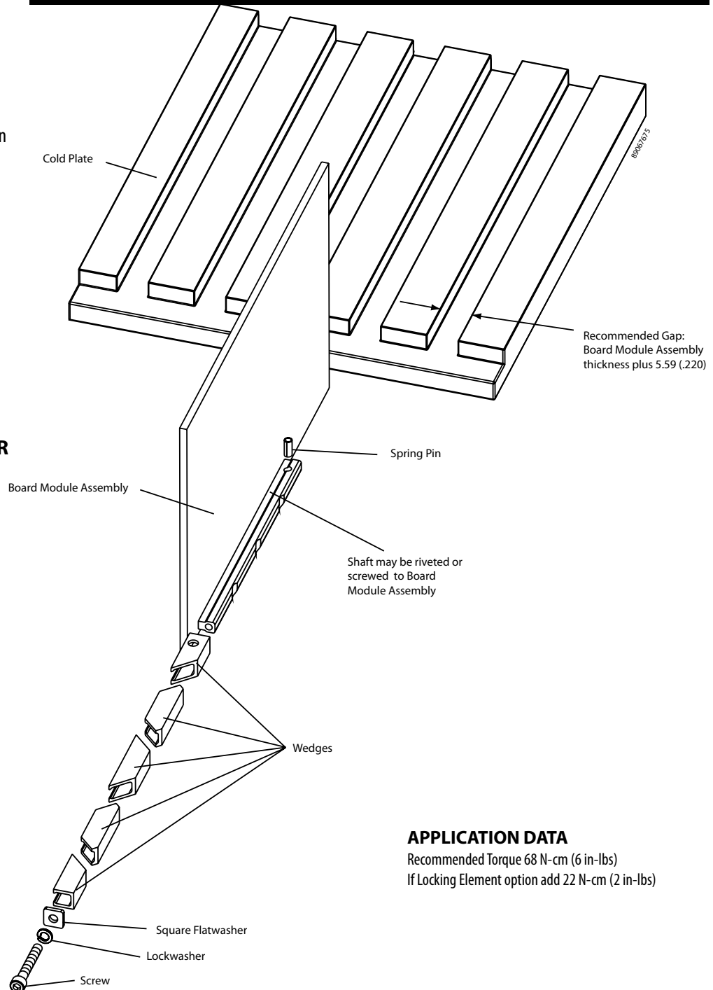
Series 267 - "Card-Lok" Retainer (narrow)
