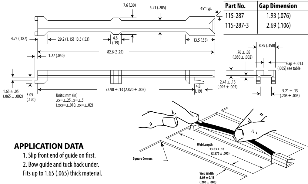
Series 115-287 - Nylon Guide
