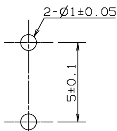
P.C.B.piercing plan
