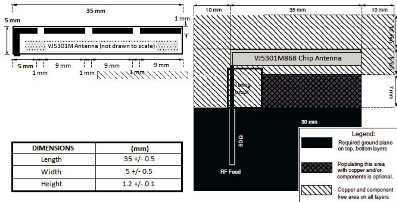
Fig. 7 - Footprint, Chip Antenna Mechanical Dimensions, and PCB Layout Dimensions of VJ5301M868
