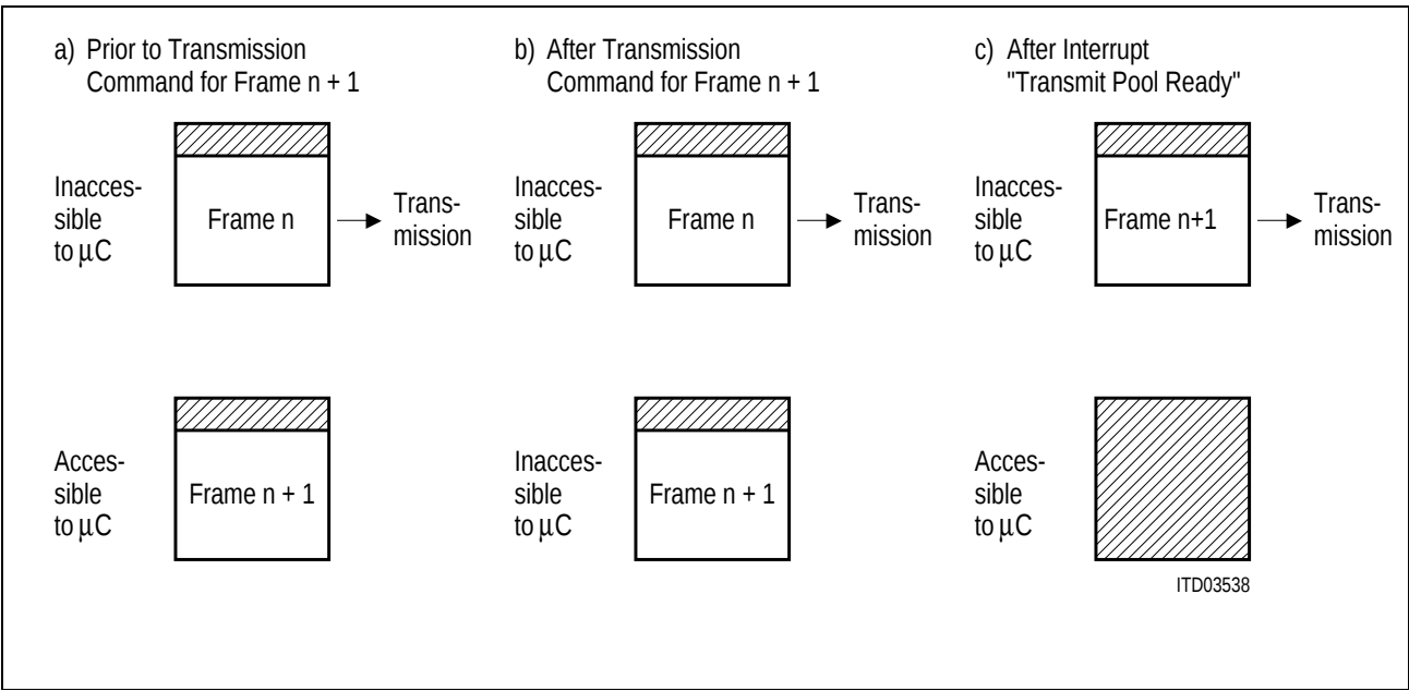
Figure 11 Transmit FIFO
