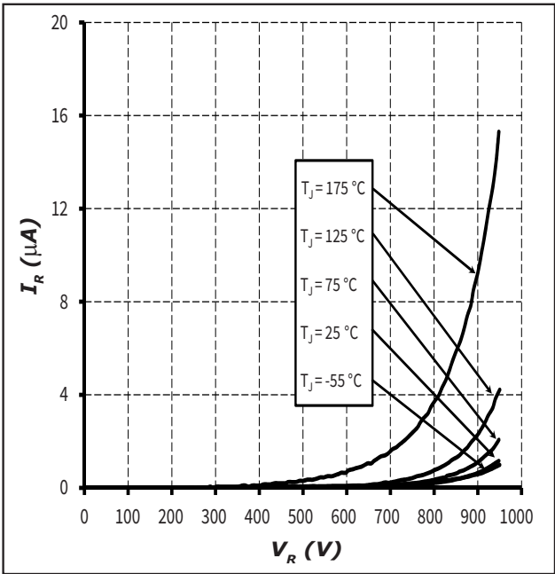
Figure 2. Reverse Characteristics
