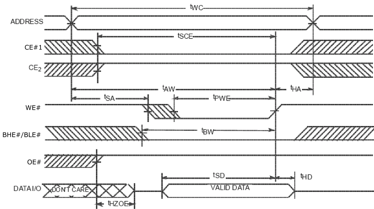
Figure 28. Write Cycle I ( \overline{WE\#} Controlled)
