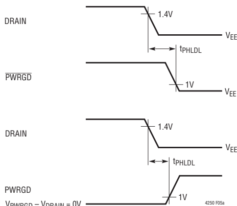
Figure 5a. DRAIN to \overline{\text{PWRGD}}/\text{PWRGD} Timing
