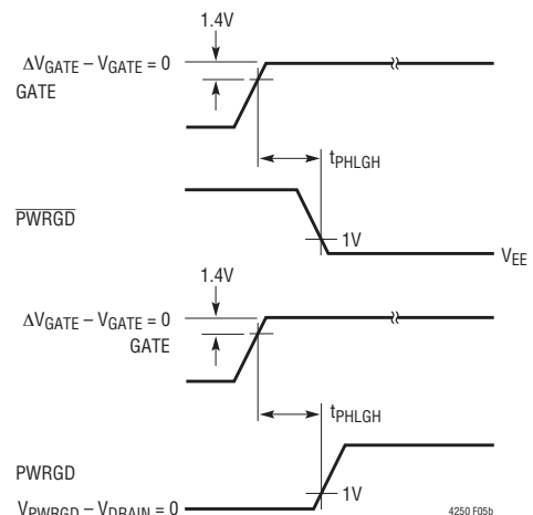
Figure 5b. GATE to \overline{\text{PWRGD}}/\text{PWRGD} Timing
