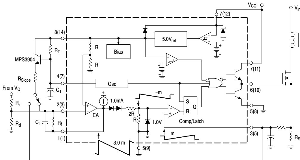
Figure 33. Slope Compensation
