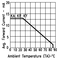
Fig 4. Max. Average Forward Current vs. Ambient Temperature.
