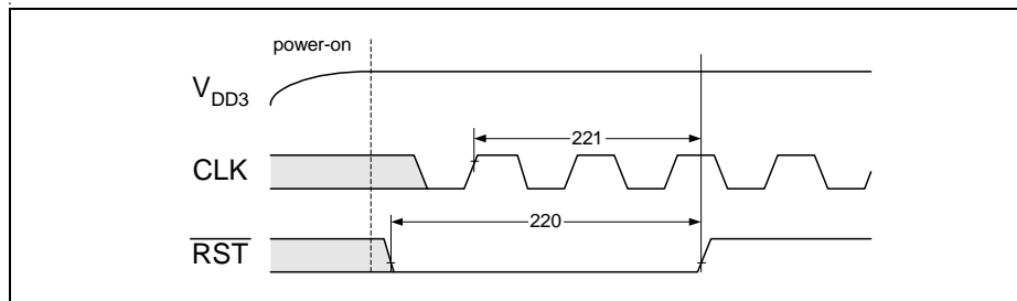
Figure 9-36 Reset Timing
