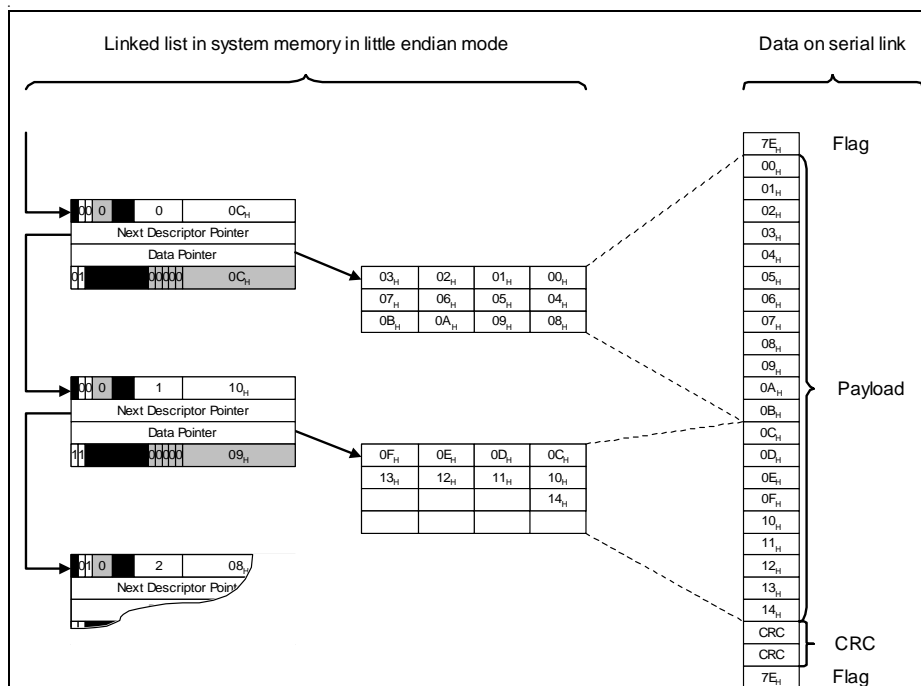
Figure 4-6 Descriptor Structure
