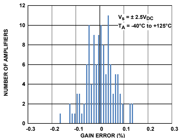
FIGURE 7. PGIA GAIN ERROR DISTRIBUTION, G = 100
