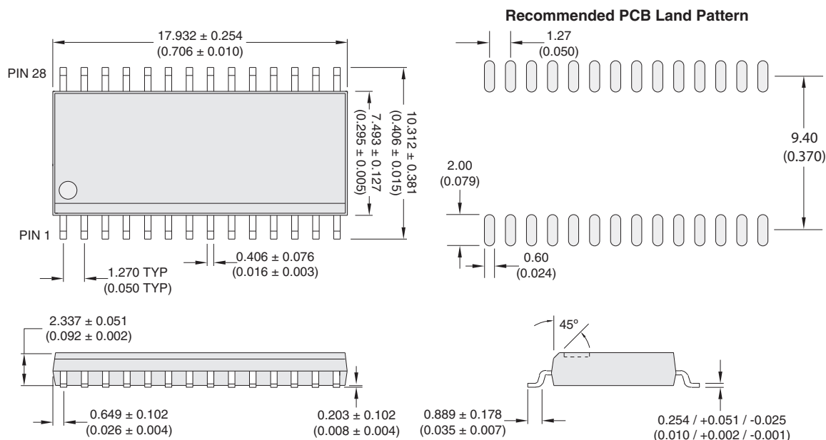
CPC7695Bx Package
