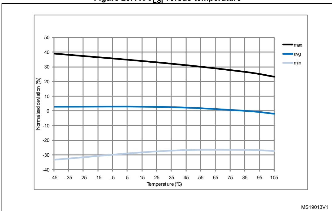
Figure 28. \text{ACC}_{\text{LSI}} versus temperature
