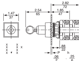
Key Operator Selector Switch
