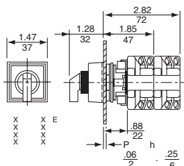
Selector Switch Operator Non-Illuminated
