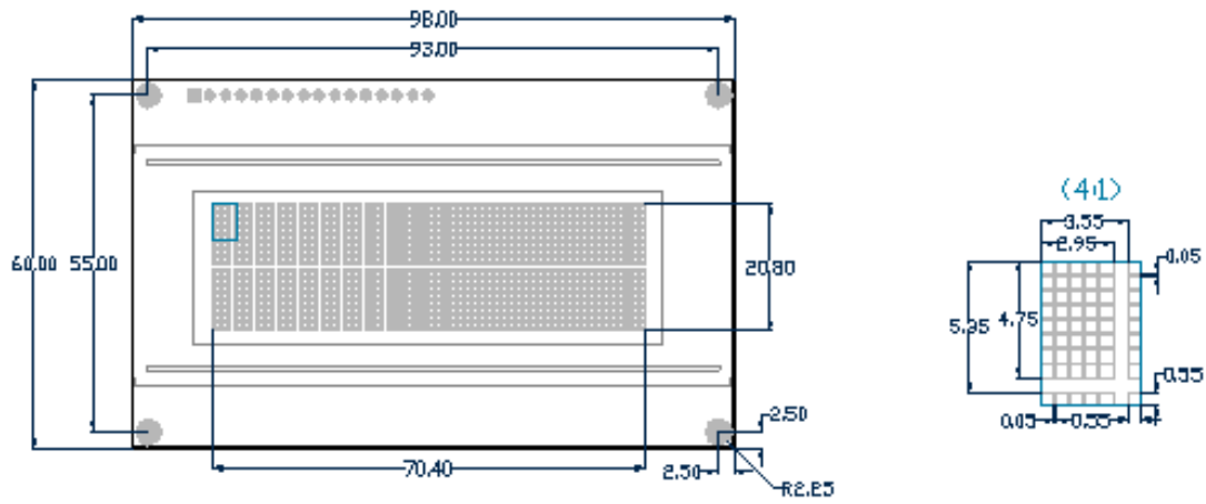
Figure 23: LCD Dimensional Drawing
