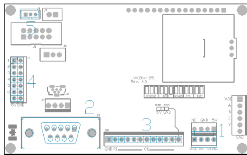
Figure 3: Standard Connections
