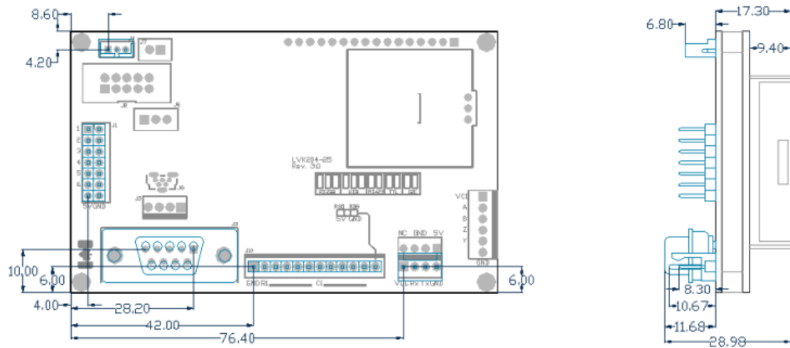
Figure 24: LVK204-25 Dimensional Drawing
