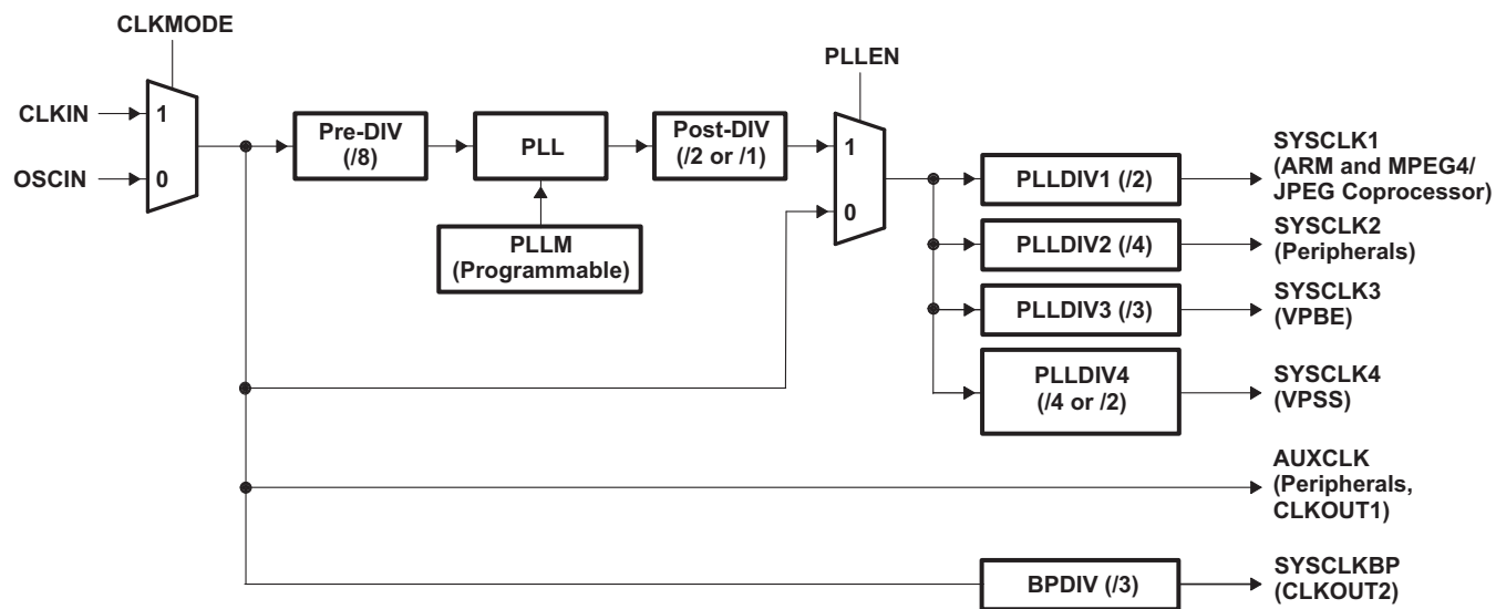
Figure 3-3. PLLC1 Configuration in DM355
