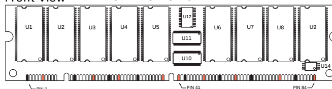
Front View Low Profile PCB
