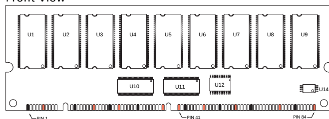
Front View Standard PCB
