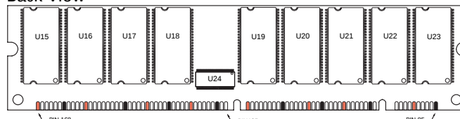
Back View
