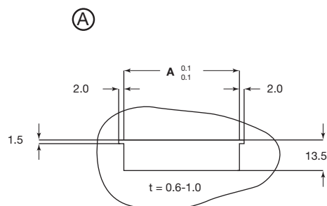
Dimension A = No. of Pos. x 5 + 9.0 mm
