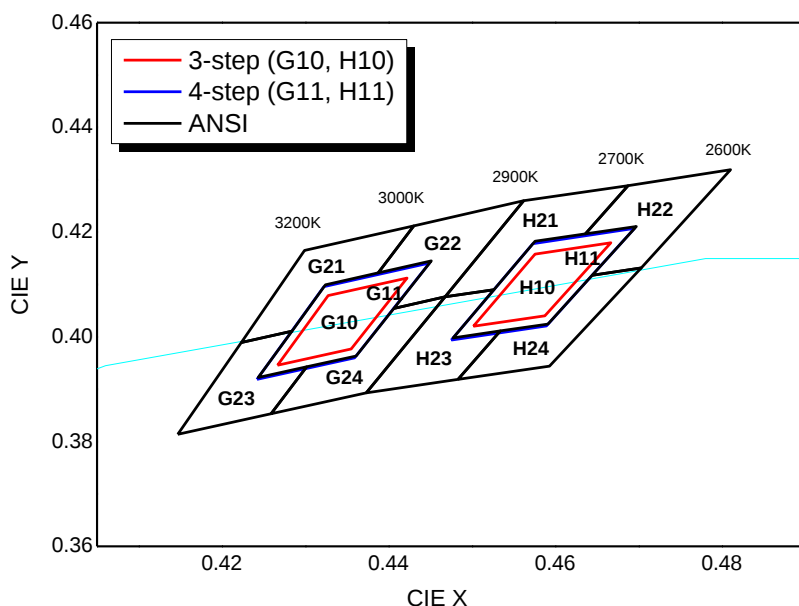
CIE Chromaticity Diagram (Warm white), Ta=25℃, IF=350mA
