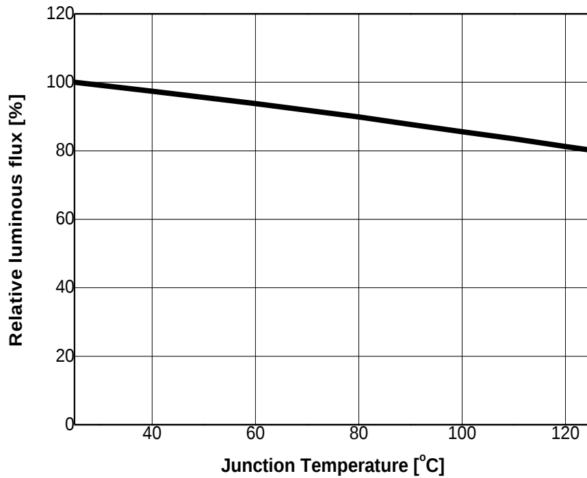
Fig 6. Relative Light Output vs. Junction Temperature, I_F=350\text{mA}
