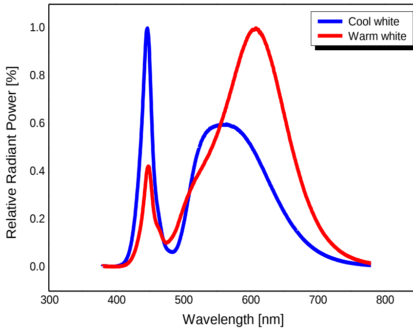
Fig 1. Color Spectrum, T_a = 25^{\circ}\text{C} , I_F = 350\text{mA} , RH30%
