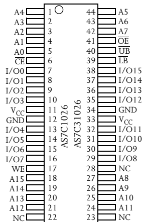
44-Pin SOJ (400 mil), TSOP 2
