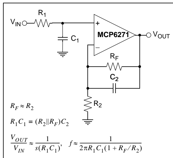
FIGURE 4-9: Non-Inverting Integrator.
