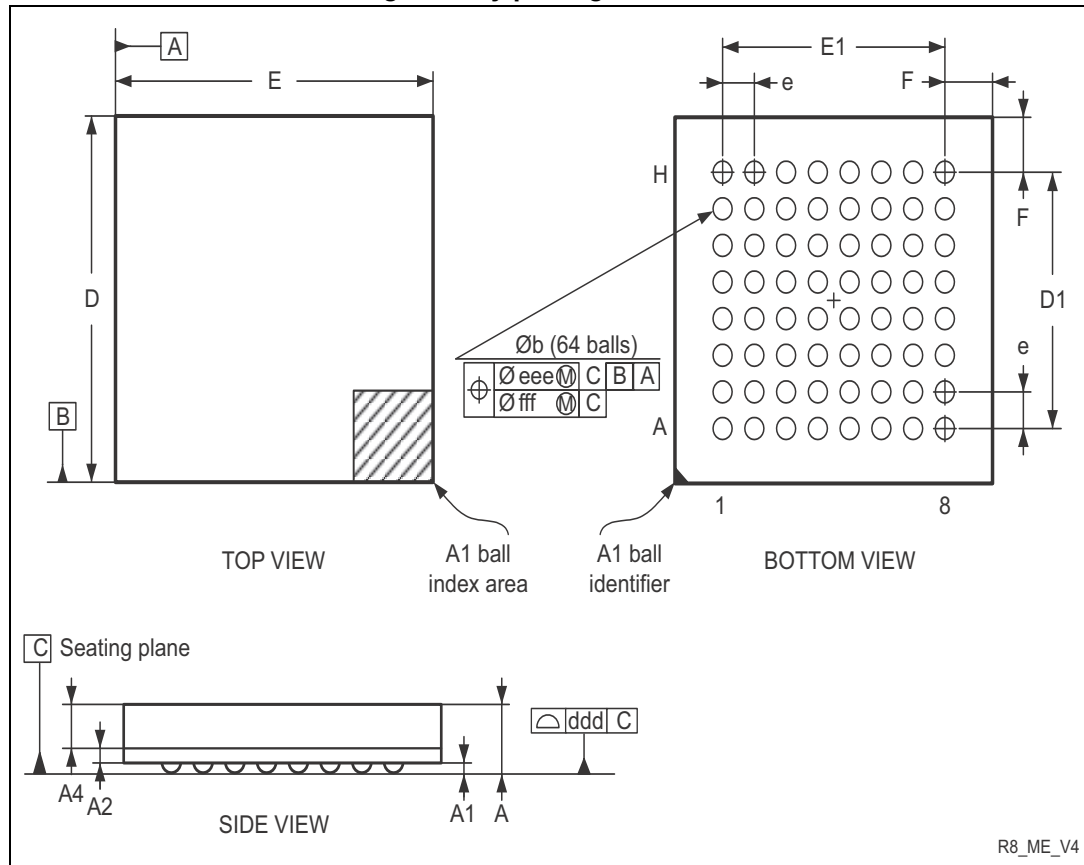
Figure 47. TFBGA64 – 64-ball, 5 x 5 mm, 0.5 mm pitch thin profile fine pitch ball grid array package outline
