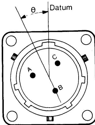
Alternative position of insert with socket contacts (Ø counter clockwise)
