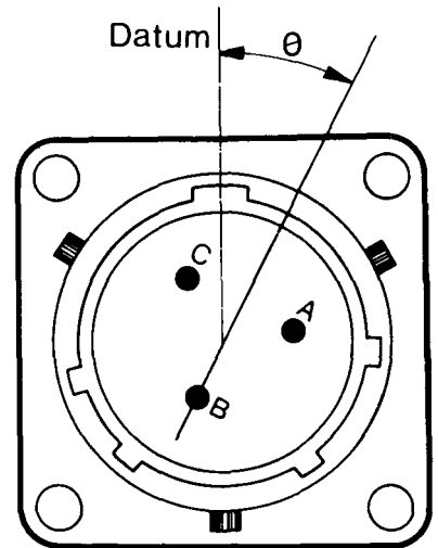
Alternate position of insert with pin contacts (Ø clockwise)
