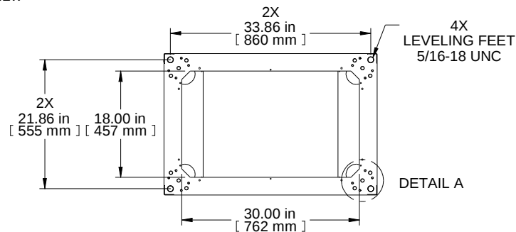
BOTTOM VIEW BOTTOM OPENING
