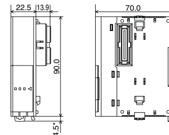
FC4A-HPH1
