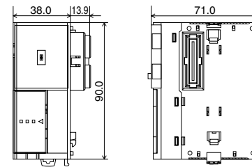
FC4A-HPH1
