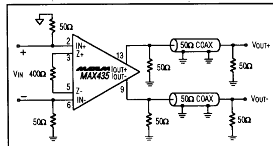
Figure 3. MAX435 Coaxial Cable Driving Circuit
