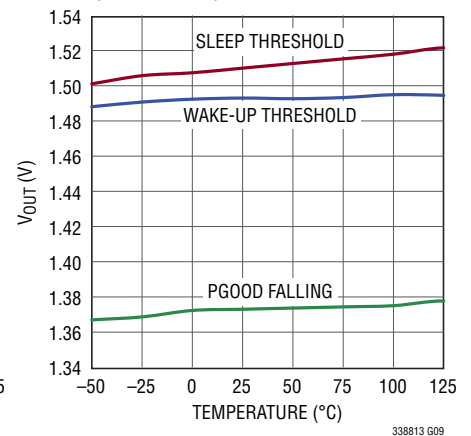
1.5V Output vs Temperature (LTC3388-1)
