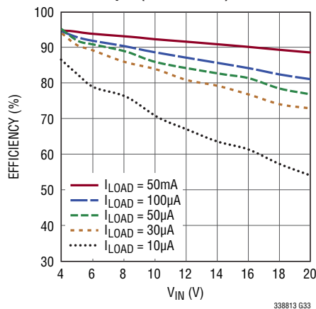
Efficiency vs V_{IN} for V_{OUT} = 3.3V , L = 100\mu H (LTC3388-3)
