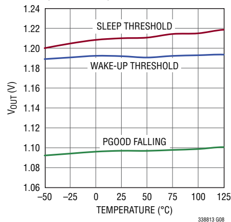
1.2V Output vs Temperature (LTC3388-1)
