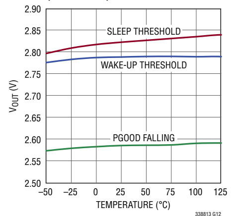
2.8V Output vs Temperature (LTC3388-3)
