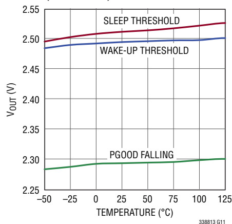
2.5V Output vs Temperature (LTC3388-1)
