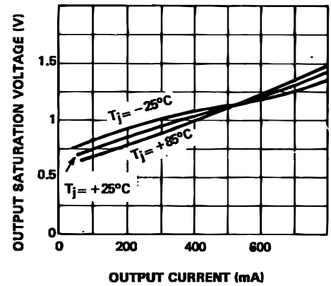
OUTPUT SATURATION VOLTAGE.
