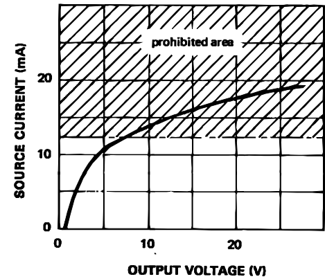
ALARM OUTPUT CURRENT SOURCE (normal operation).
