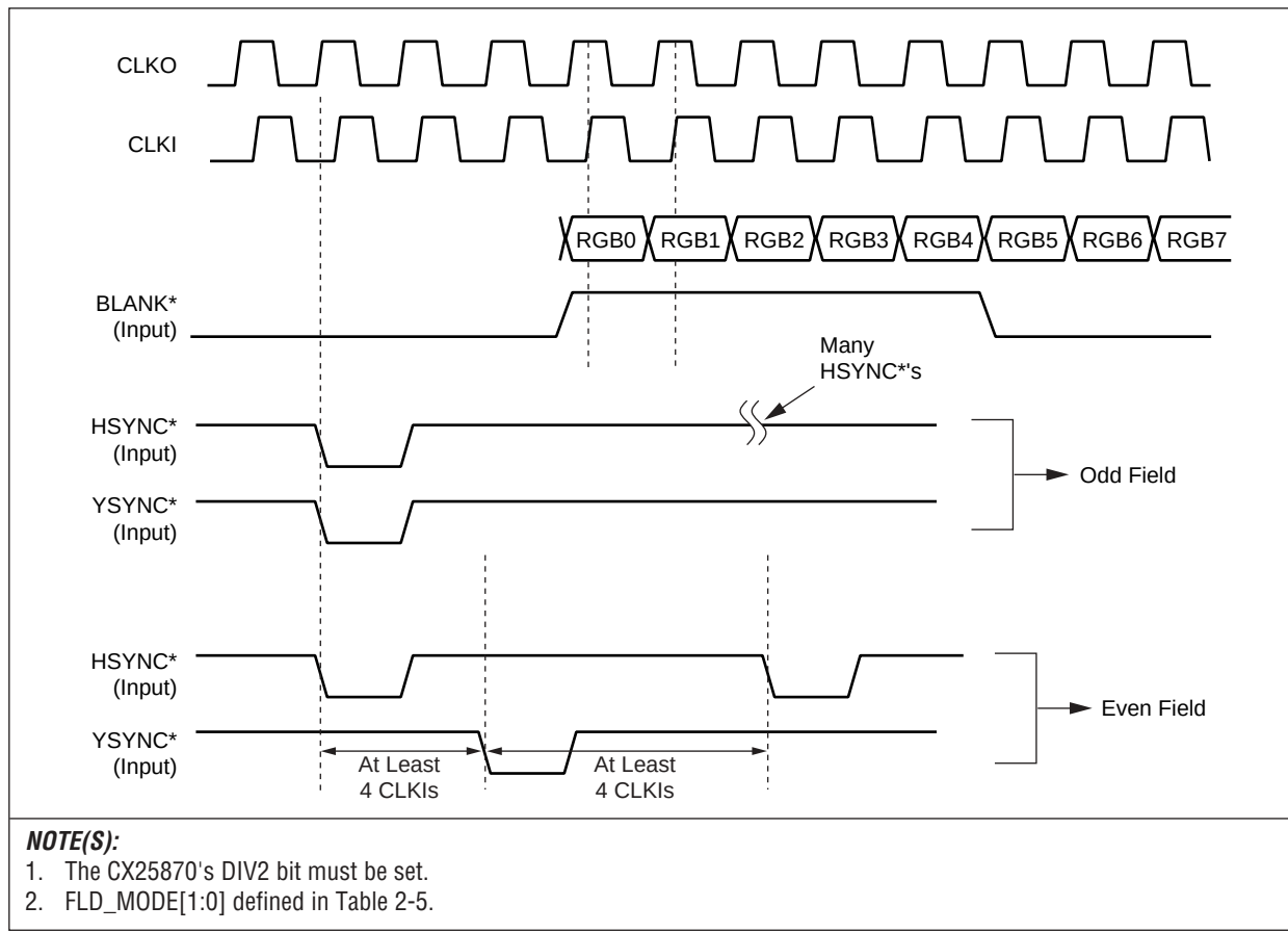
Figure 4-6. Slave Interface Timing Relationship/Interlaced Nonmultiplexed RGB Input (FLD_MODE = 10 – Default)
